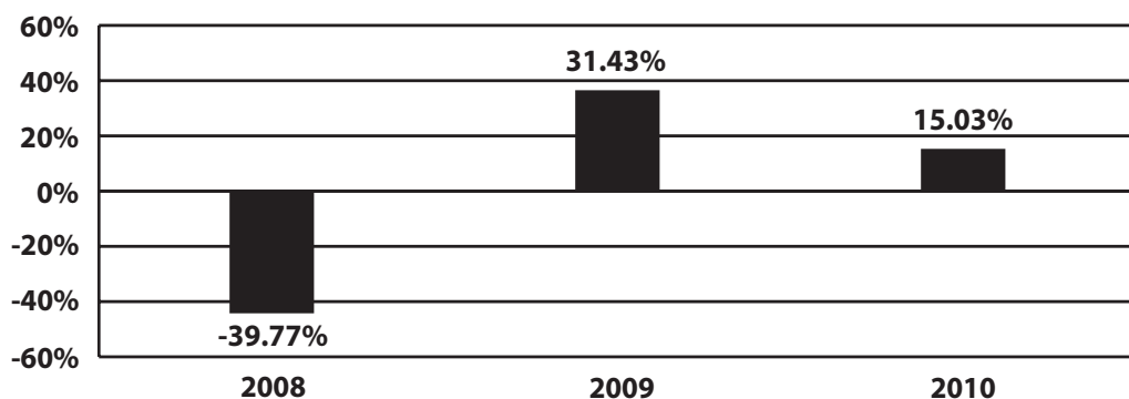
Calendar Year Total Return as of 12/31
